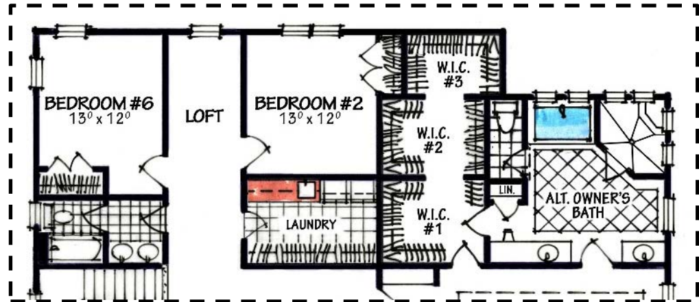
OPT. 6 TH BEDROOM & ALT. OWNER'S BATH PARTIAL PLAN
