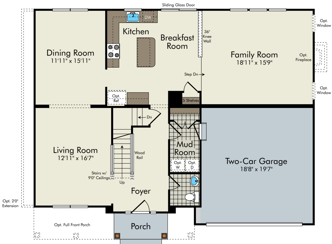
First Floor w/ Opt. 2'0" Full Rear Extension
