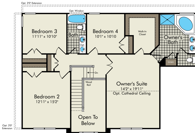
Standard Second Floor
