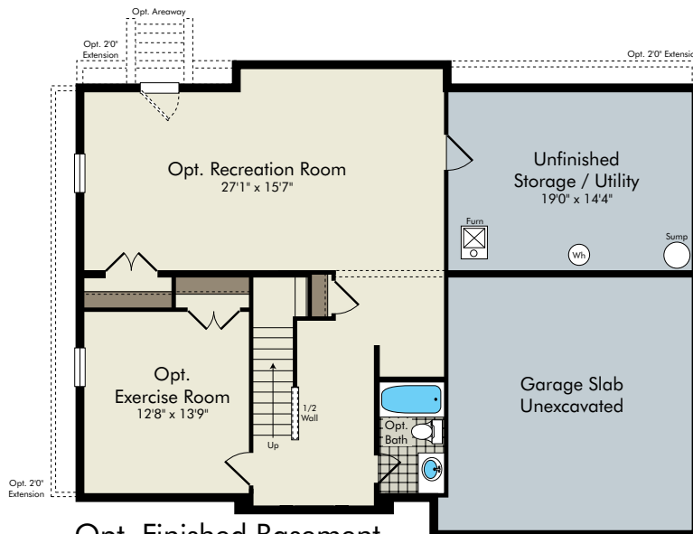
Opt. Finished Basement
