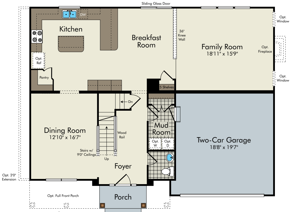
First Floor w/ Opt. 2'0" Full Rear Extension & Alternate Kitchen
