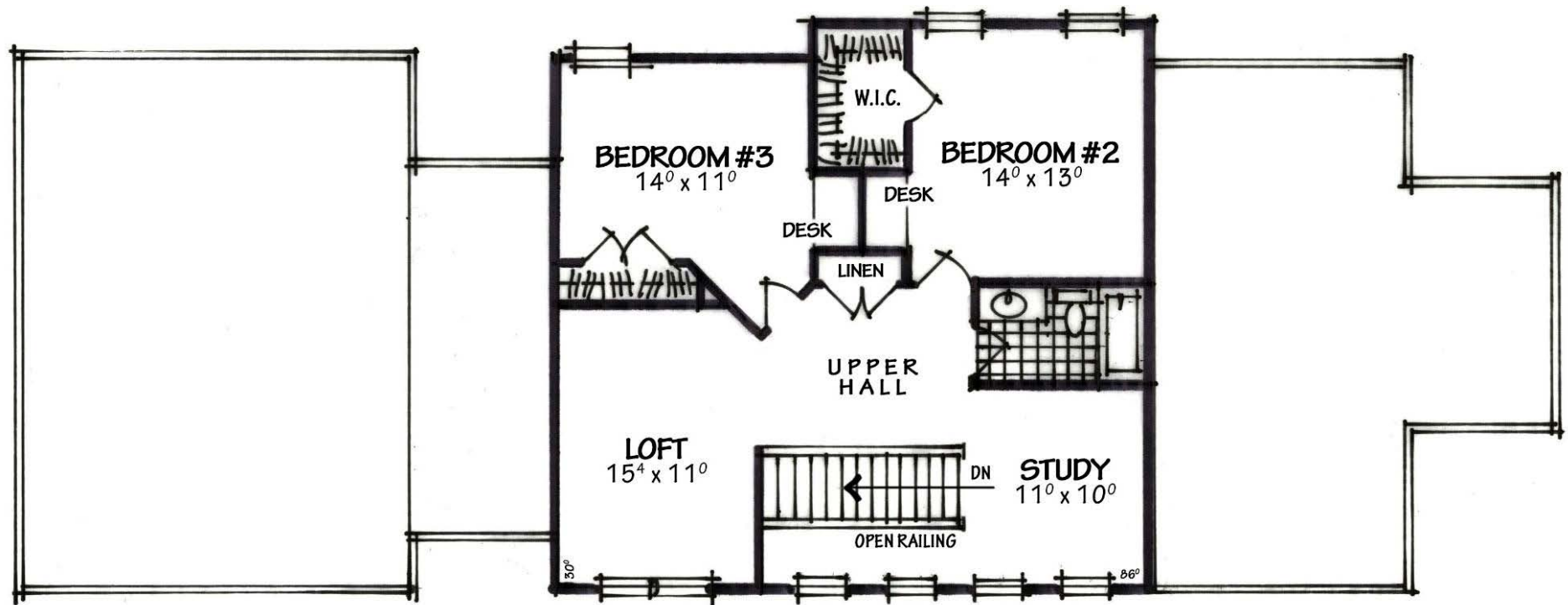
SECOND FLOOR PLAN 1,049 S.F.
